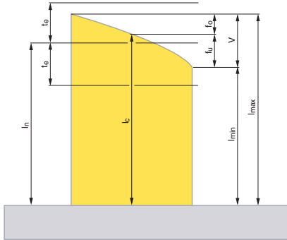
Nominal length l_n ; Central length l_c ; Variation v with f_0 and f_1 ; Limit deviations t_e at any point proceeding from the nominal length.
